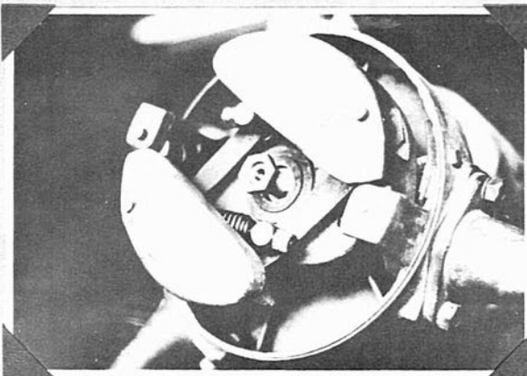
PHOTO 11. Rurallite Governor - Showing Flyball Weights
