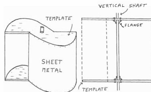
Figure 4 Savonius Wing Assembly.
