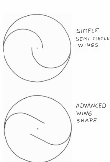
Figure 1 Simple and Advanced Shapes for Savonius Rotor Wings.
