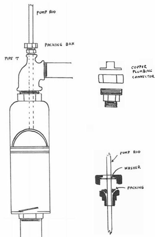
Figure 5 Inexpensive packing box for piston pump.
