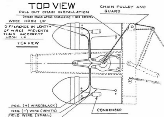
FIGURE B Jacobs Twin-Motor 1500 Watt - 32 Volt - Model 15
